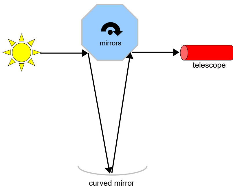
Illustration 3: Michelson's apparatus.
