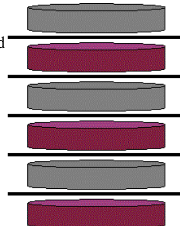
Figure 2: A simple battery made up of two dissimilar metals separated by cloth soaked in acid.
